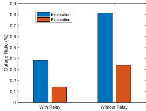
Fig. 6. Outage time percentage considering maximum available beams for service
