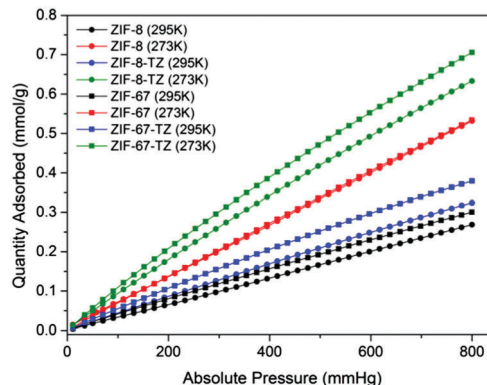
Fig. 4 CH_4 adsorption isotherms at 273 and 295 K.
