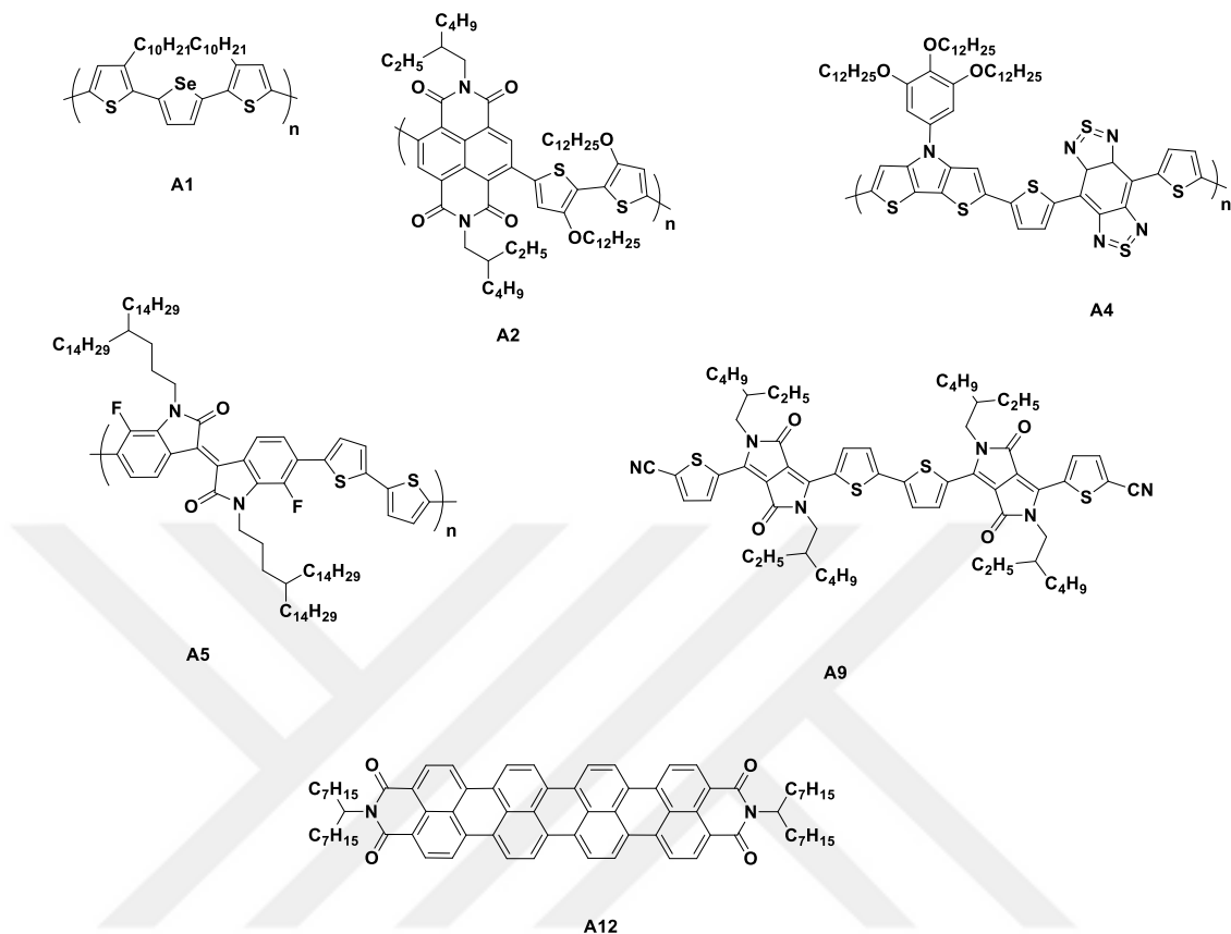
Figure 1.5.3 Chemical structures of ambipolar polymeric semiconductors.
