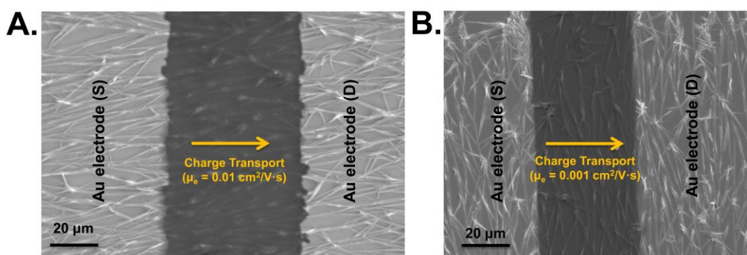
Figure 3.2.5.4.5. Top-view SEM images of OTFT devices fabricated via solution shearing of BDY-4T-BDY with source-drain electrodes deposited perpendicular (A) and parallel (B) to the major fiber alignment direction.
