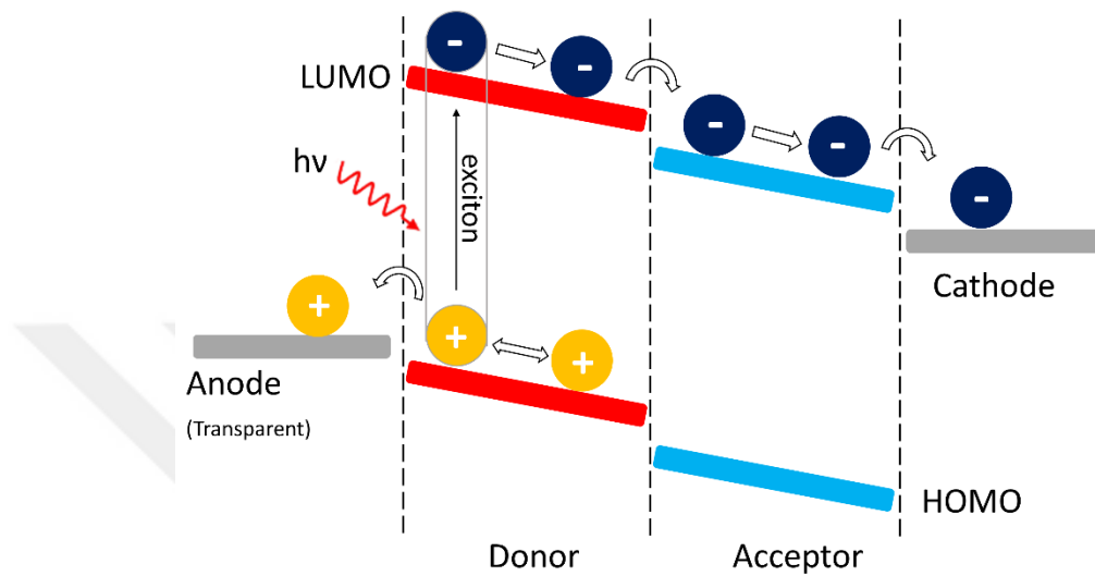
Figure 1.4.2.1 Simplified schematic showing the principal internal processes taking place in OPVs.
