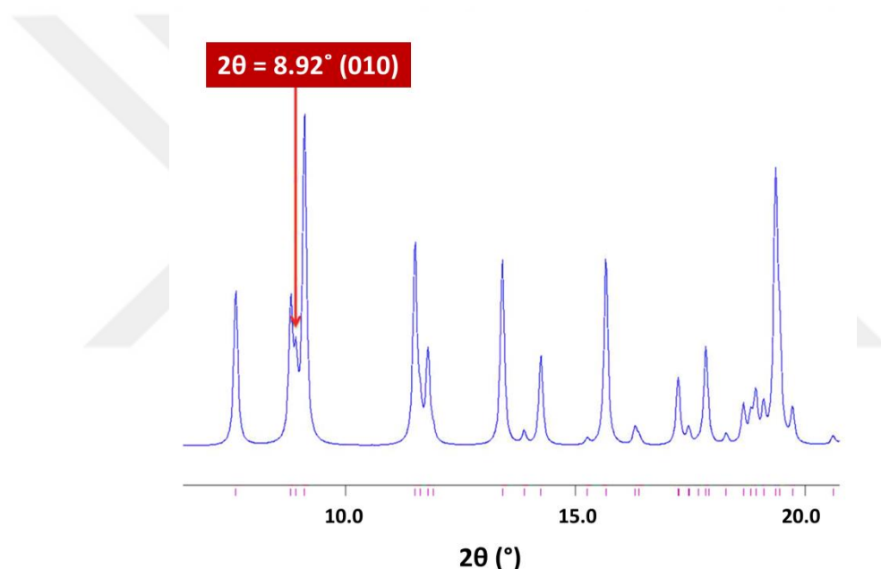
Figure 3.3.4.3.1. Simulated XRD powder pattern of BDY-PhAc-BDY with the selected matching peak at 2\theta = 8.92^\circ corresponding to (010) diffraction plane.
