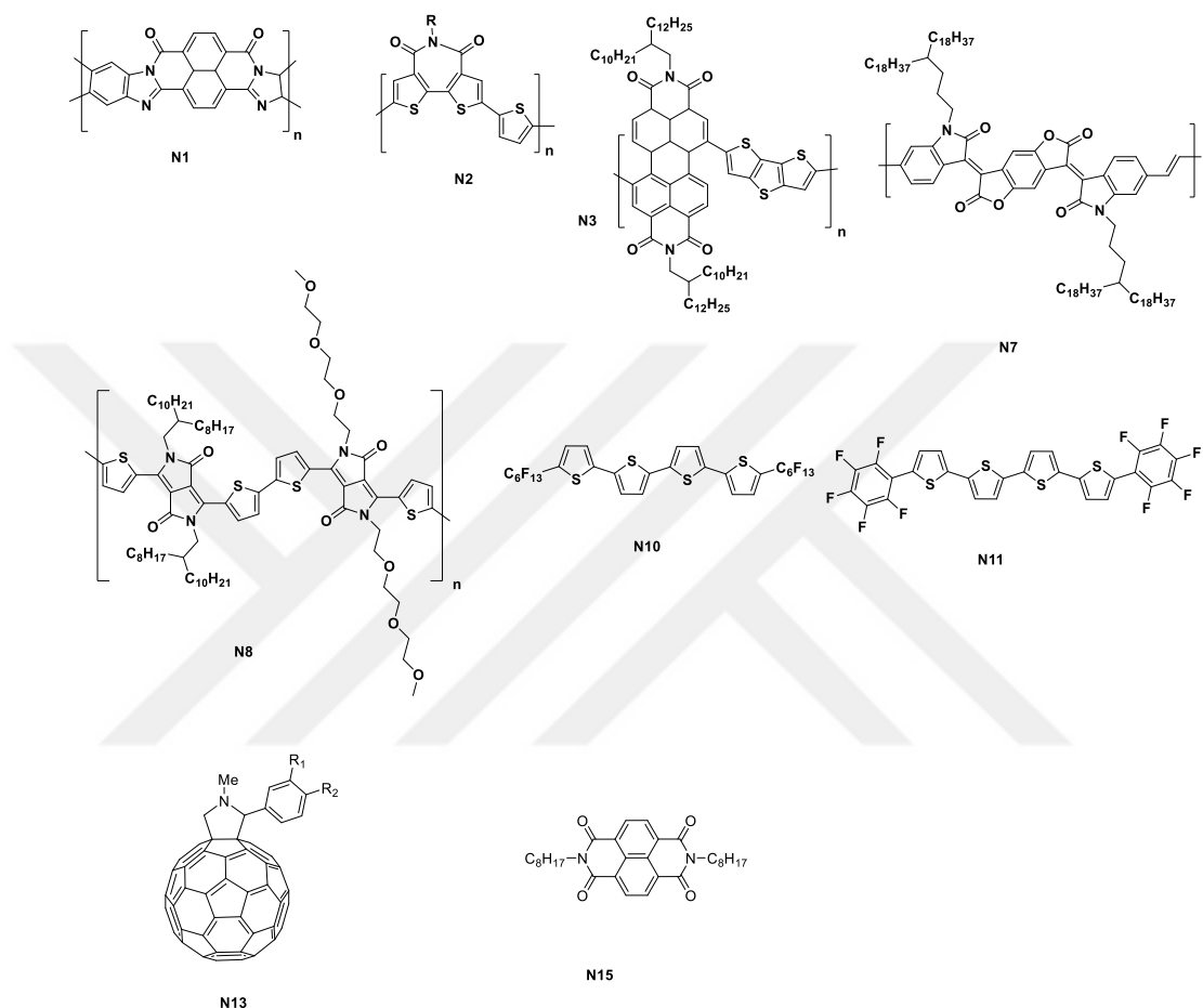
Figure 1.5.2 Chemical structures of n -channel polymeric semiconductors.
