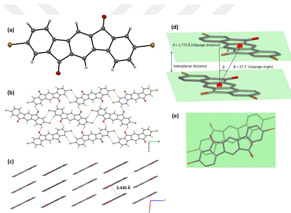
Figure 2.3.4 (a) ORTEP drawings of the crystal structure (50% probability level). (b) Perspective view of 2D network via -\text{CH} \cdots \text{Br} (blue dashed lines) and -\text{CH} \cdots \text{O} (red dashed lines) contacts. (c) Perspective view of brick-wall packing arrangement with an interplanar distance of 3.430 Å. (d) and (e) Representations of pairs of indeno[1,2-b]fluorene-6,12-dione molecules arranged in a slipped \pi -stacked fashion (The red, grey, brown, and white coloured atoms represent O, C, Br, and H, respectively).
