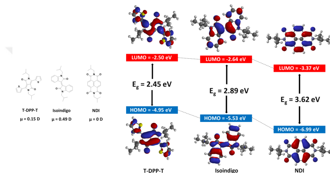
Figure 4.3.1.2 The chemical structures, molecular dipole moments ( \mu ), HOMO/LUMO energies and the corresponding pictorial orbital representations for commonly known \pi -acceptor building blocks dithienyldiketopyrrolopyrrole (T-DPP-T), isoindigo, and naphthalenediimide (NDI).
