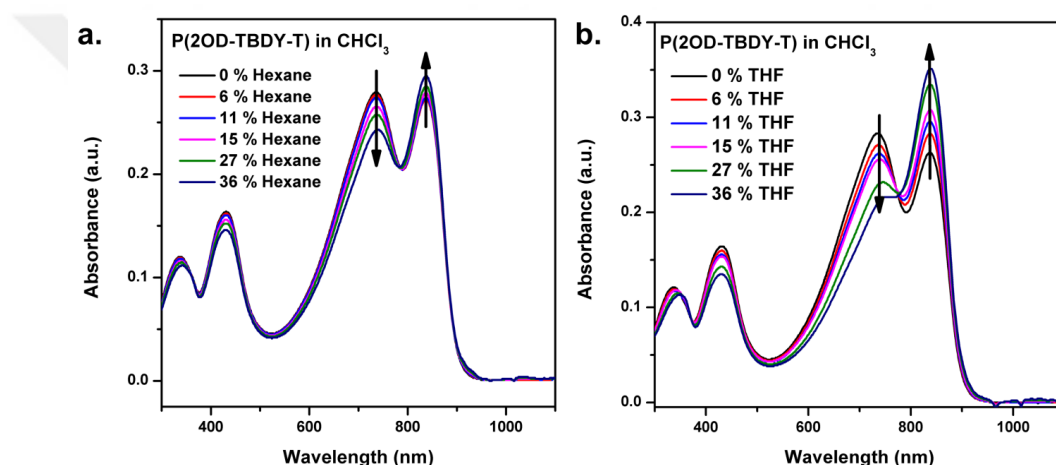
Figure 4.3.2.4 Solvent-dependent optical absorption spectra of P(2OD-TBDY-T) chloroform–hexane (a) and chloroform-THF (b) mixtures at room temperature starting in pure chloroform (black lines) and successively increasing the volume fraction of non-solvent/bad solvent.
