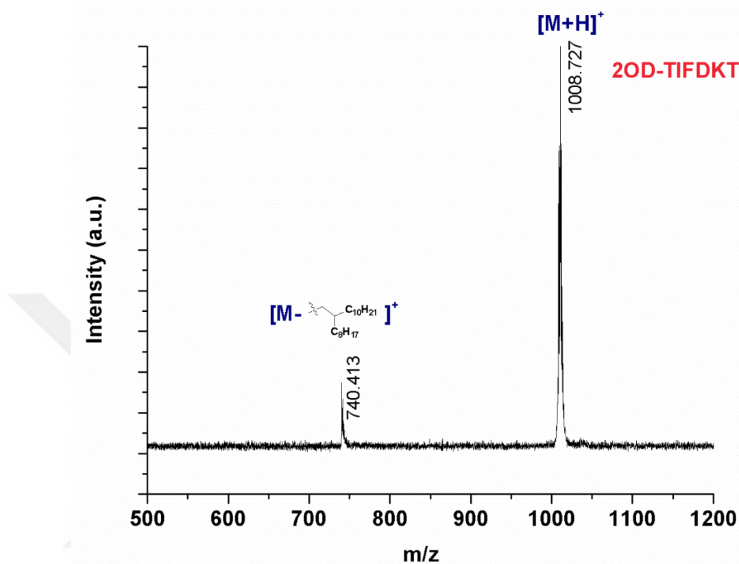
Figure 2.2.3.6.3 Positive ion and linear mode MALDI TOF-MS spectrum of 2OD-TIFDKT .
