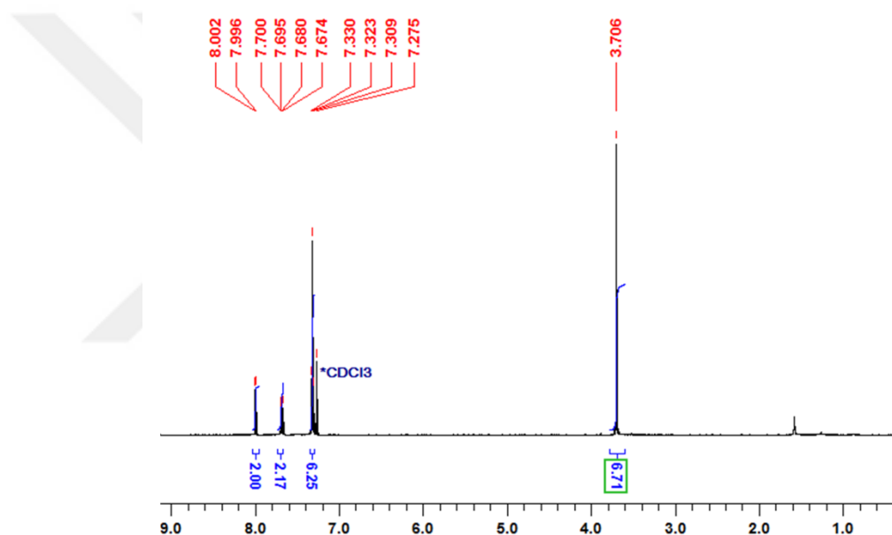
Fig. 2. 1.3.2 1 H NMR spectra of compound 1 in CDCl 3 at room temperature.
