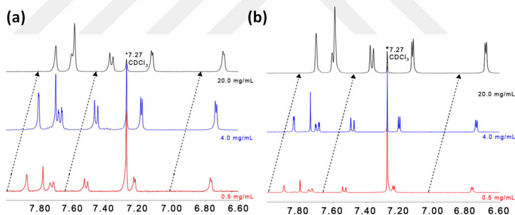
Figure 2.3.1.2 The concentration-dependent 1 H NMR spectra of 2EH-TIFDKT (a) and 2OD-TIFDKT (b) in CDCl 3 .
