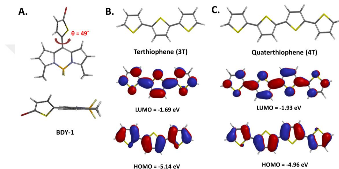
Figure 3.2.5.1.2. Optimized molecular geometries of BDY-1 (A), 2,2':5',2''-terthiophene (B) and 2,2':5',2'':5'',2'''-quaterthiophene (C) showing computed HOMO and LUMO energy levels and topographical representations (DFT, B3LYP/6-31G**).
