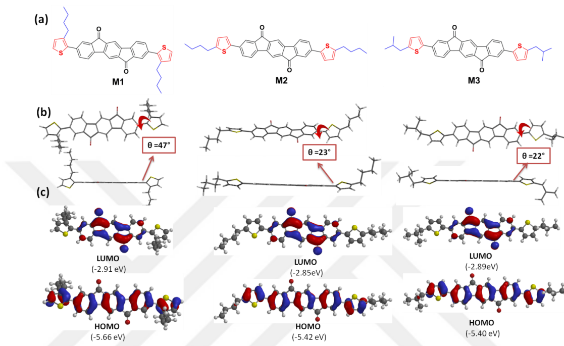
Figure 2.3.1.1 a) Chemical structures of the model compounds M1 , M2 , and M3 . b) Optimized molecular geometries showing inter-ring dihedral angles. c) Computed HOMO and LUMO energy levels, and topographical representations (DFT, B3LYP/6-31G**) )
