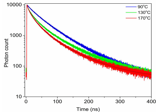
Fig. 2. Time correlated single photon count decays for alloyed core/shell In(Zn)P/ZnS quantum dots as a function of core growth temperature.
